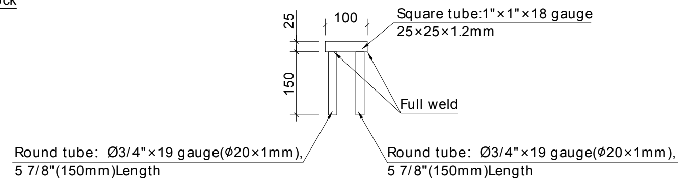
Top connector-2
