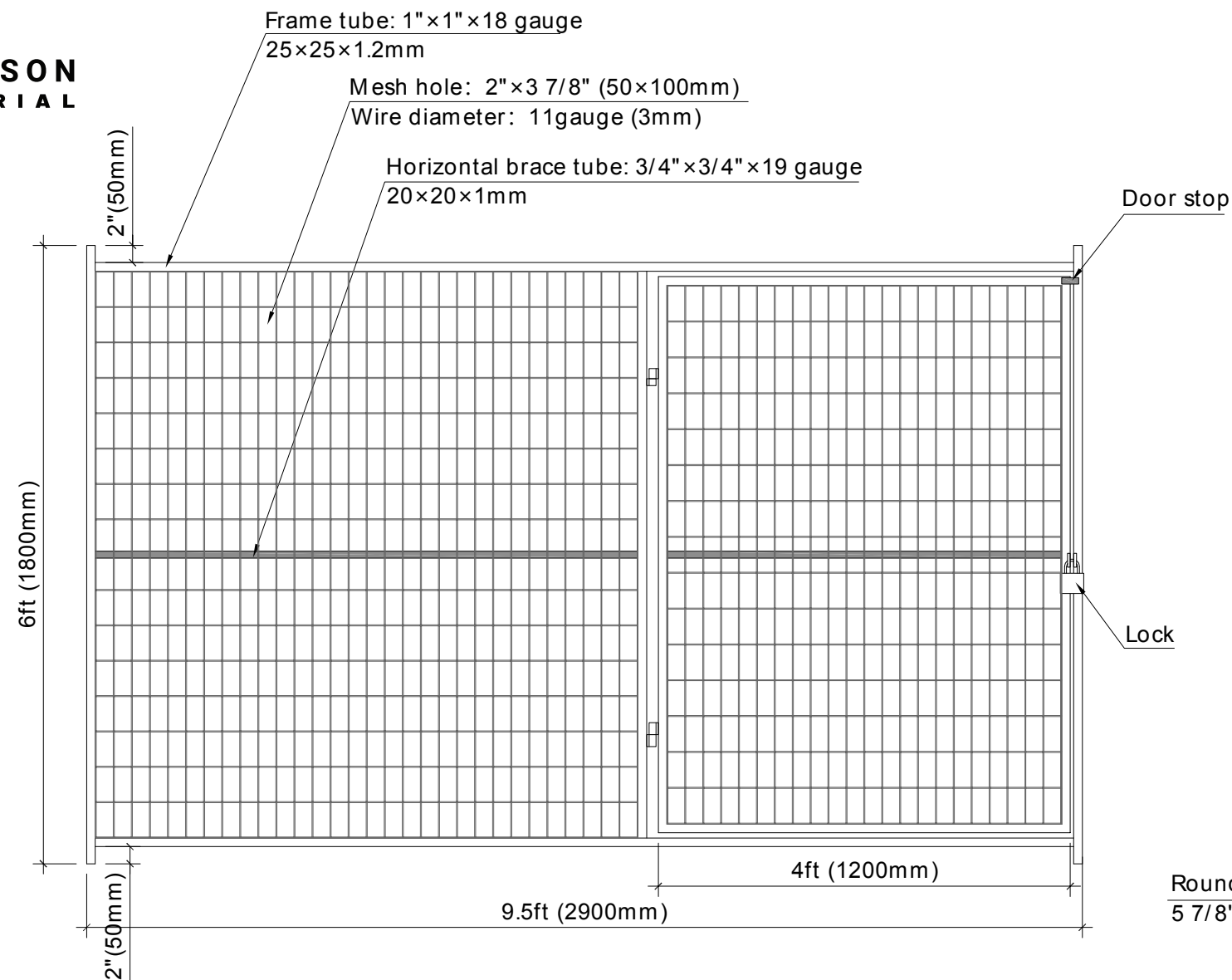
Front view
