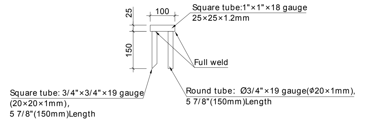
Top connector-1
