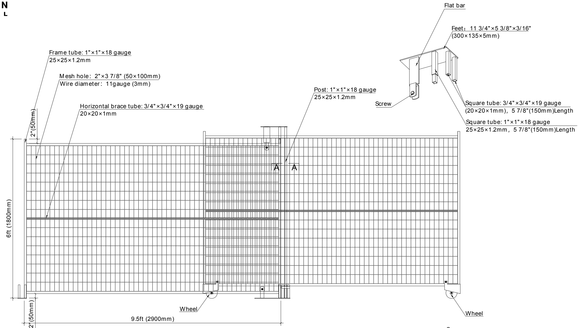
Front view
