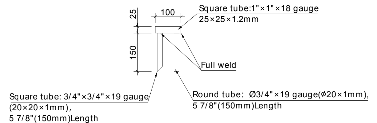
Top connector-1
